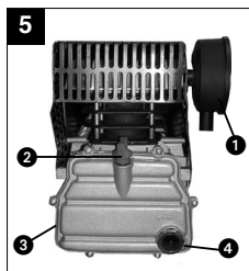
4 Schauglas
